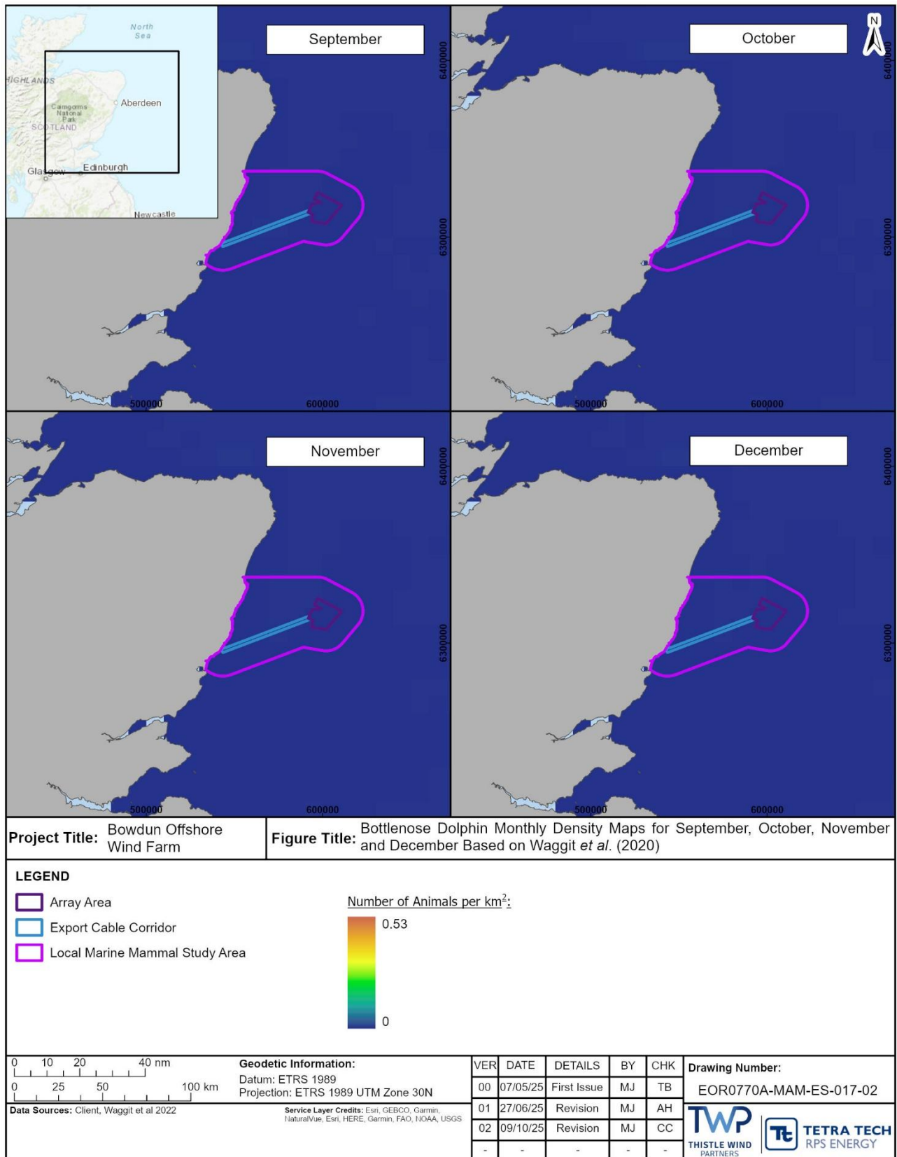
Figure 6.13: Bottlenose Dolphin Monthly Density Maps for September, October, November and December Based on Waggit et al. (2020)
