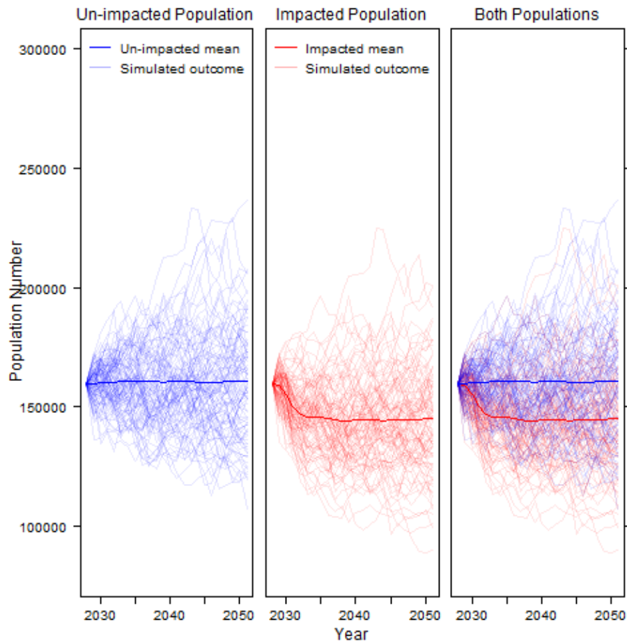
Figure 3.4: Simulated Harbour Porpoise Population Trajectories in an Un-impacted Versus Impacted Population, for Cumulative Scenario HPC2 (without Proposed Development)
