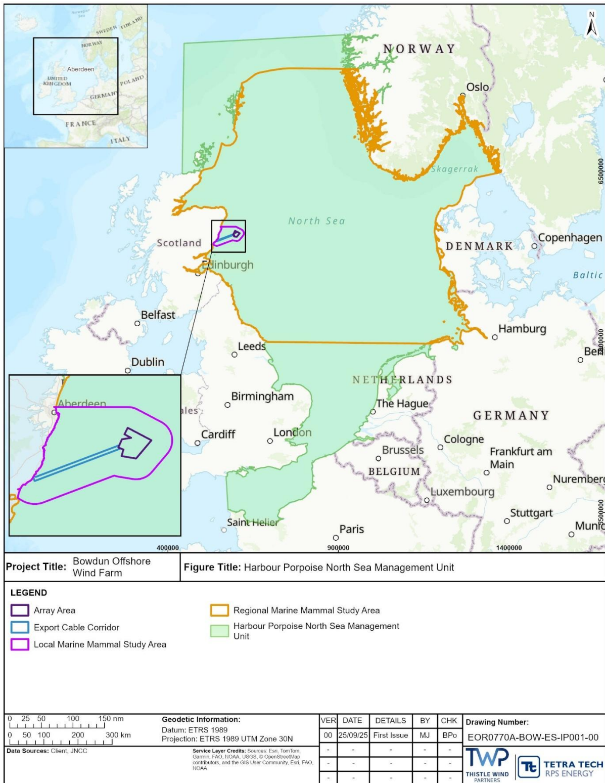
Figure 2.1: Harbour Porpoise North Sea Management Unit (IAMMWG, 2022)
