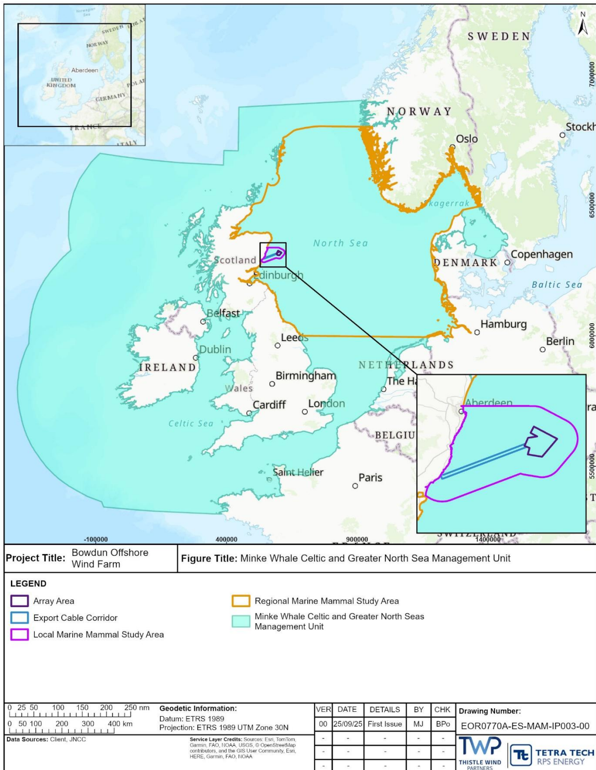
Figure 2.3: Minke Whale CGNS MU (IAMMWG, 2022)
