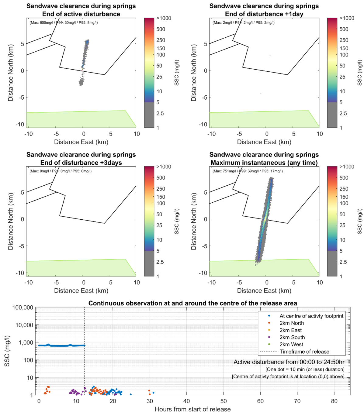
Figure A1.4: Increase in Suspended Sediment Concentration as a Result of Scenario 4: Sandwave Clearance Using a MFE in the Array Area. Mean Spring Tide
