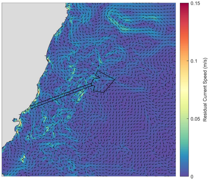
Figure D1.7: Baseline Residual Tidal Current Speed and Direction Over a Representative Spring-Neap Tidal Period
