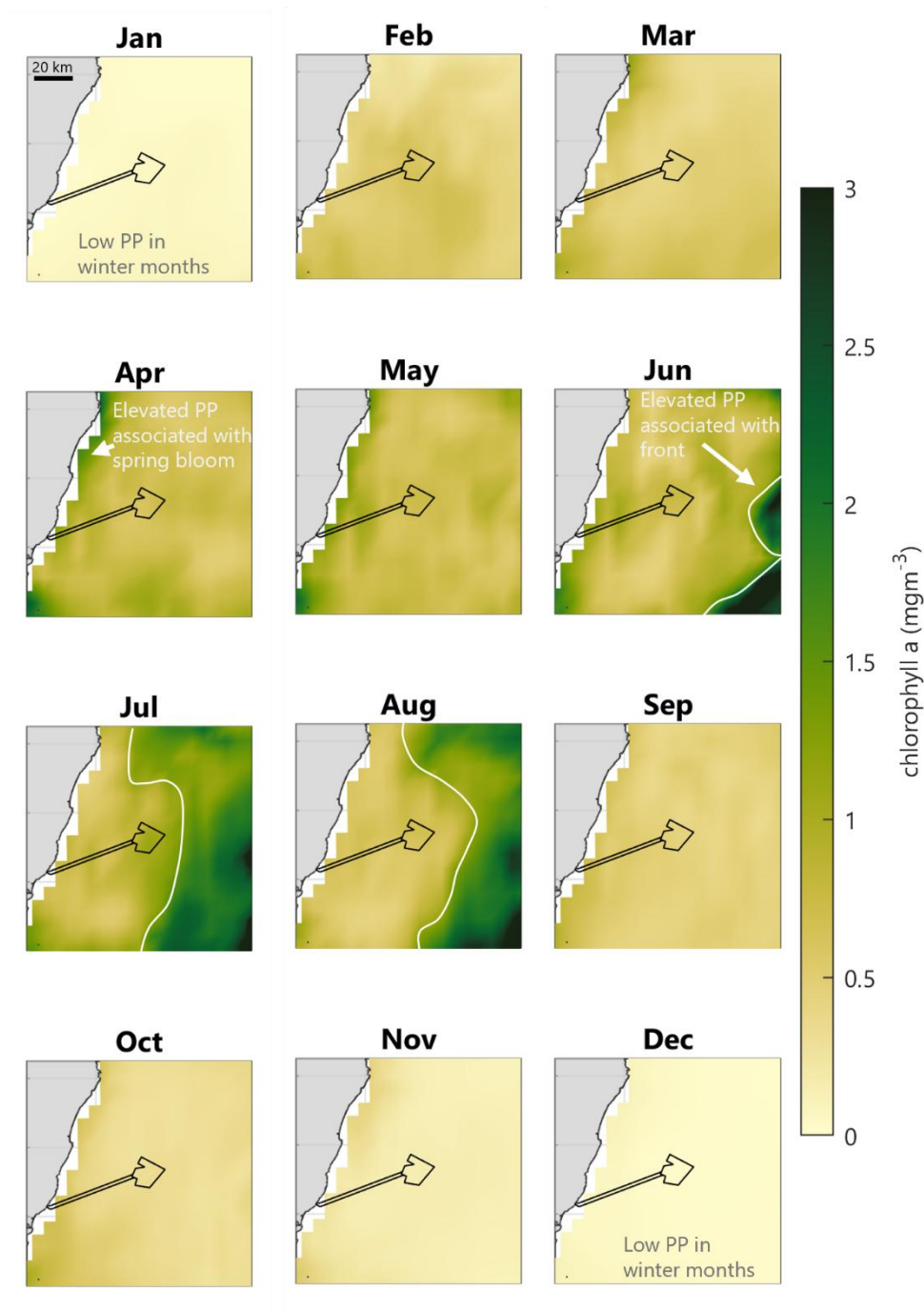
Figure 4.7: Copernicus Reanalysis Monthly Maximum Chlorophyll-a Concentration Throughout the Water Column for 2015 a Weaker Stratification Year
